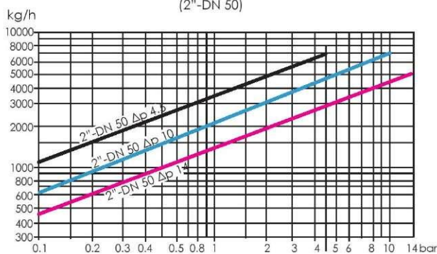
Discharge Capacities (2"-DN 50)
